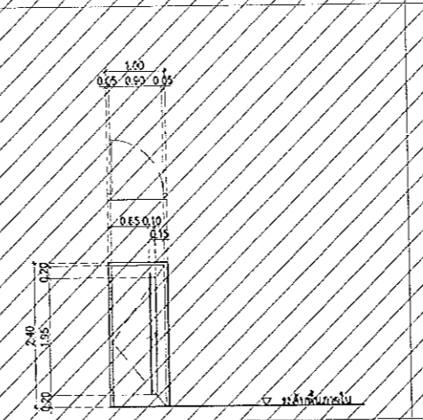
ELEVATION 03
